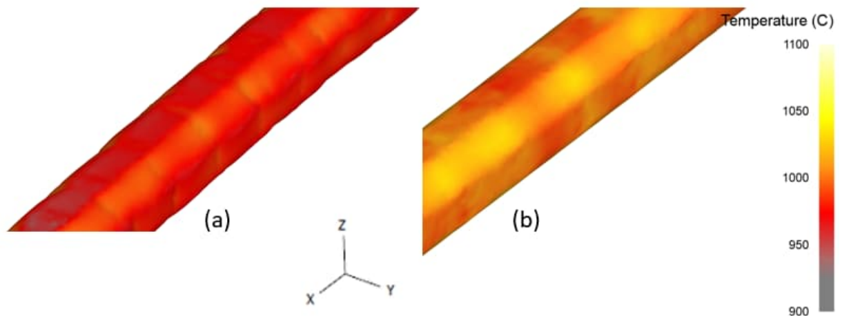
Figura 70 – Temperatura das barras “passe Oit 250 mm”: (a) 2 bigornas, 975°C (+/-25°C); (b) 4DFD, 1000°C (+/-25°C).
